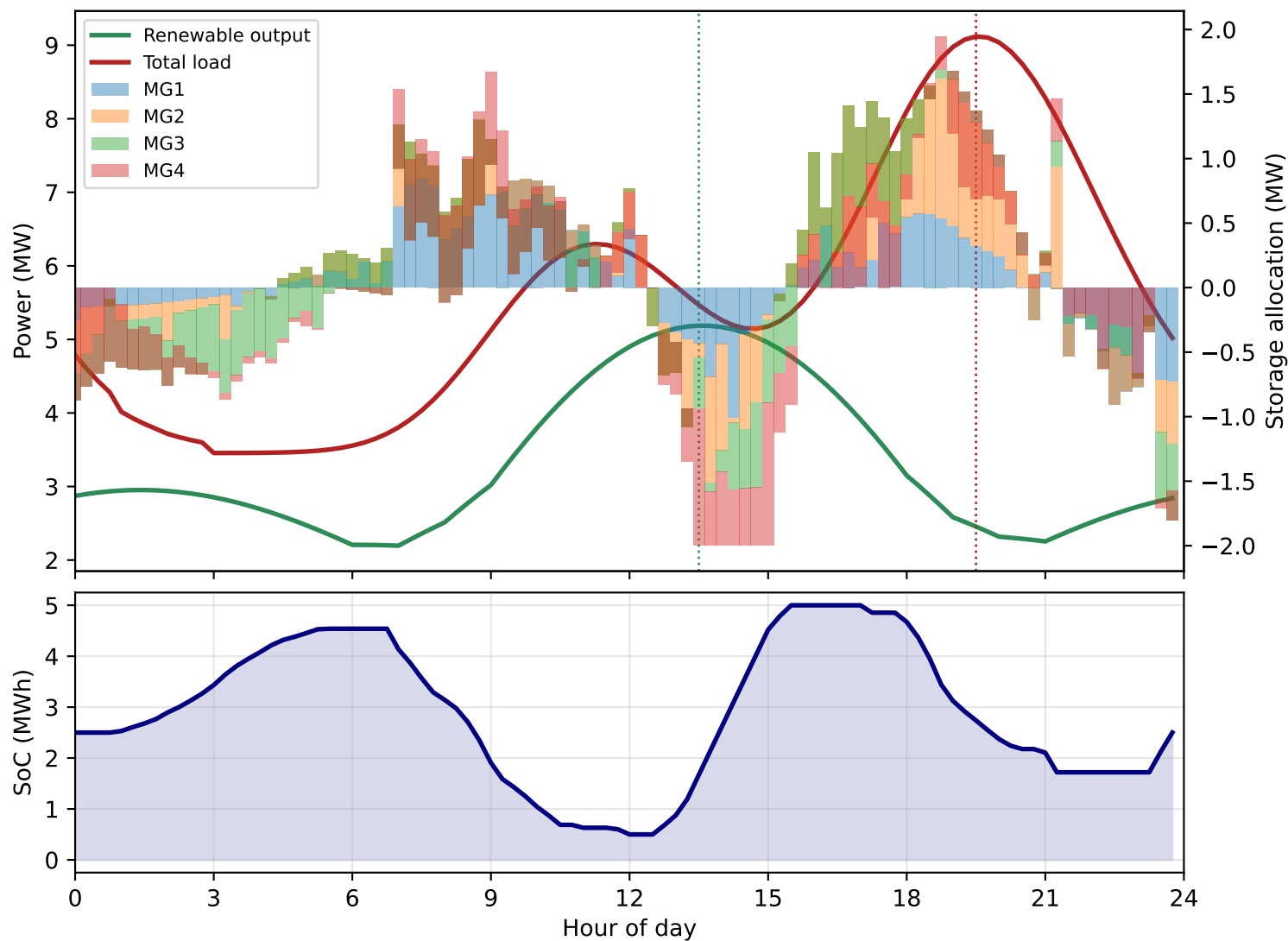
Fig2. Shared energy storage dispatch and state of charge over 24 hours
